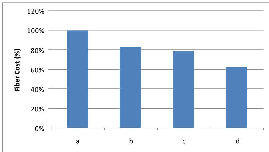
Figure 8. Fiber cost at equal panel stiffness for HMPP/carbon composites. a) 100% carbon, b) 100% carbon shell with 50/50 carbon HMPP hybrid core, c) 50/50 carbon HMPP hybrid, d) 100% carbon shell with 100% HMPP core.
