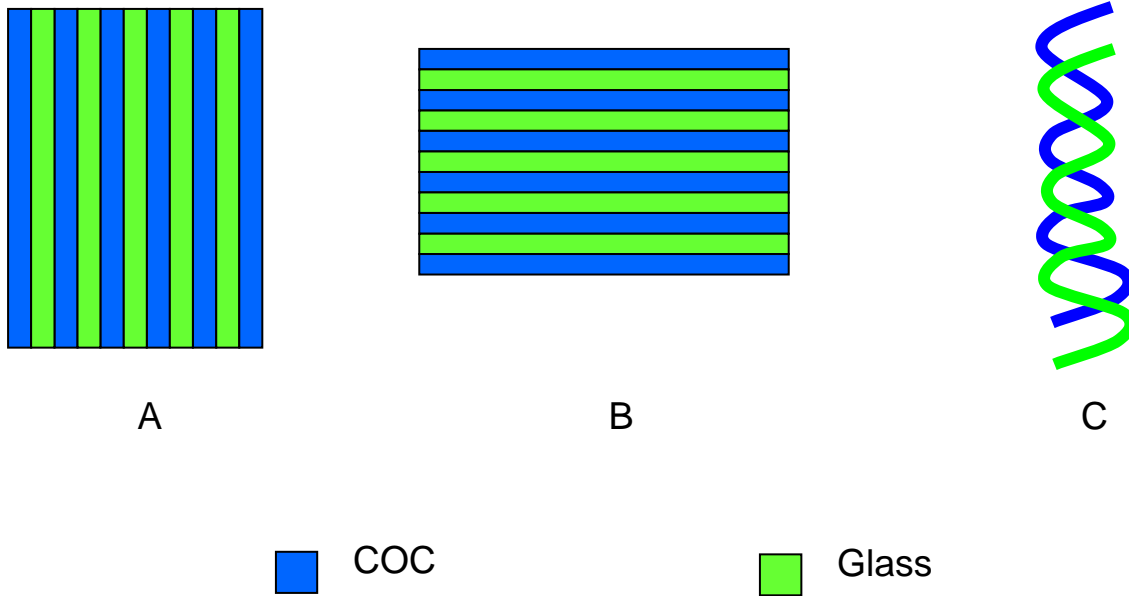
Figure 3. Ways of combining glass and COC yarns in fabric. A) Alternating warp yarns (weft not shown). B) Alternating weft yarns (warp not shown). C) Hybrid twisted or entangled yarns. D) (not pictured) Glass warp, COC weft.
