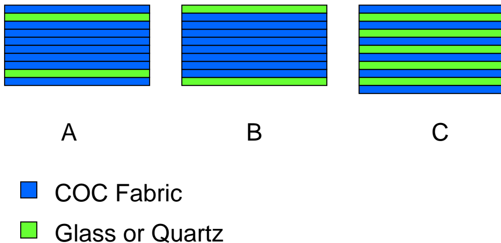
Figure 4. These schematics represent the possible configurations of Innegra and glass or quartz fabrics in hybrid composites. Advantages for each are: A: Places low dielectric fiber near the surface to minimize reflection coefficient, while retaining glass fiber just under the surface to maximize physical properties. B: Places glass farthest apart to maximize physical properties. 25 C: Evenly spaced composite materials, for the most uniform dielectric to be experienced by the traveling wave.
