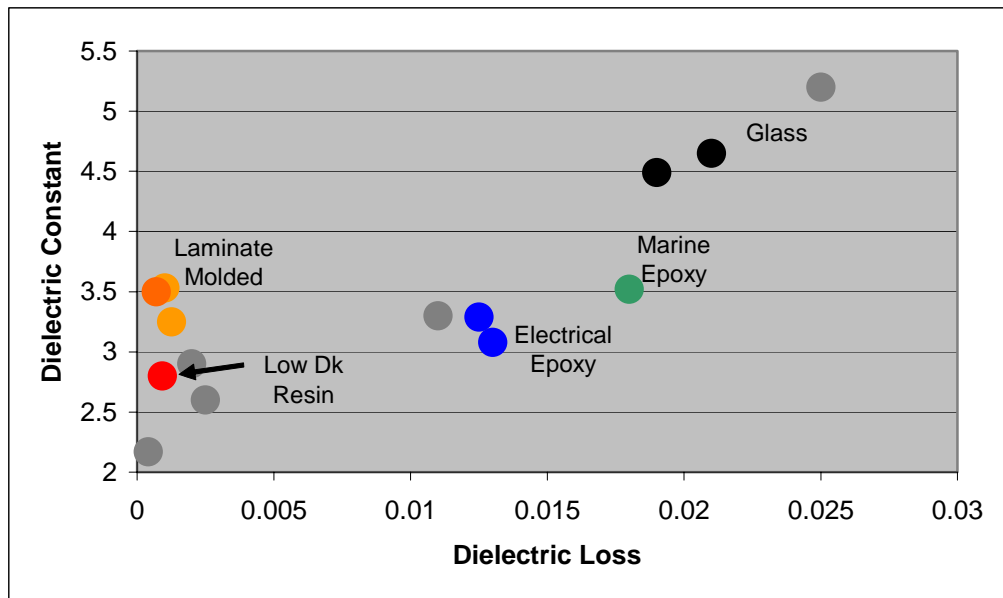
Figure 6. Dielectric constant and loss tangent of the substrates from this study, shown with the commercial substrates from Table 1 as grey ghosted spots. Low dielectric and low loss substrates are possible with the use of low dielectric yarns.
